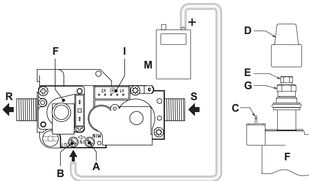
fig. 16 - Valvola gas
